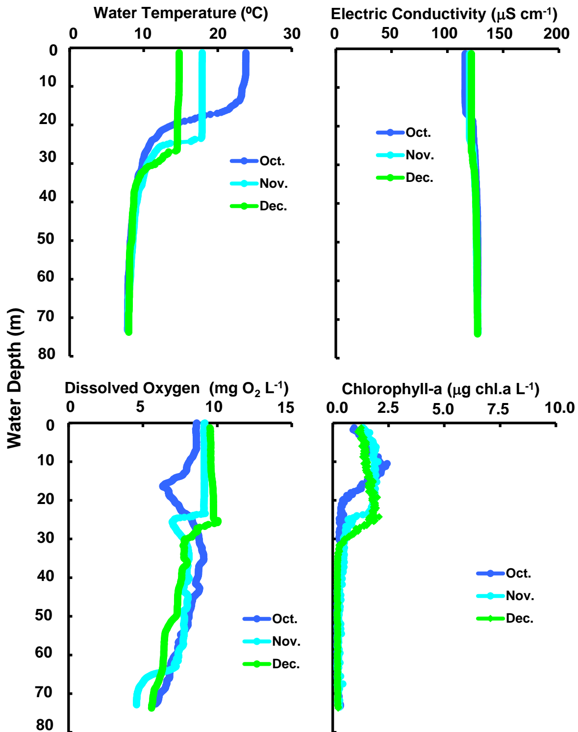
Changes of vertical distribution in water temperature, electric conductivity, dissolved oxygen concn., chlorophyll-a amount at Stn.le-1 in the north basin of Lake Biwa from October to December 2022.
