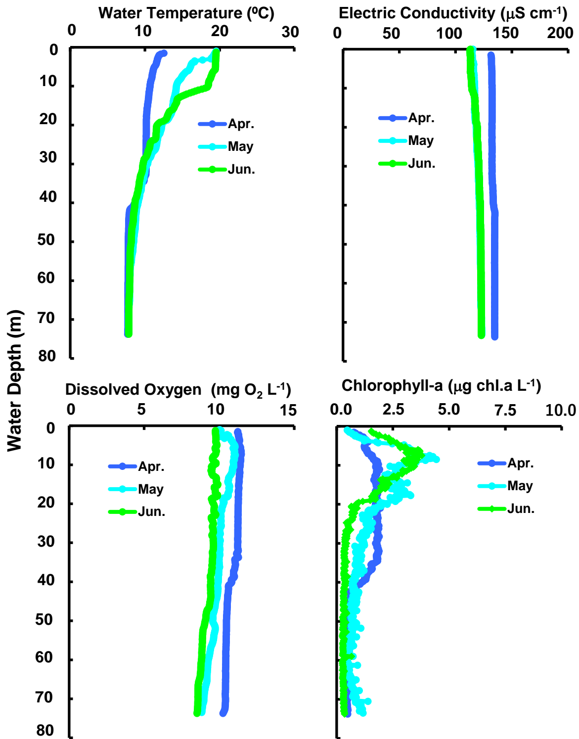
Changes of vertical distribution in water temperature, electric conductivity, dissolved oxygen concn., chlorophyll-a amount at Stn. 1e-1 in the north basin of Lake Biwa from April to June 2023.
