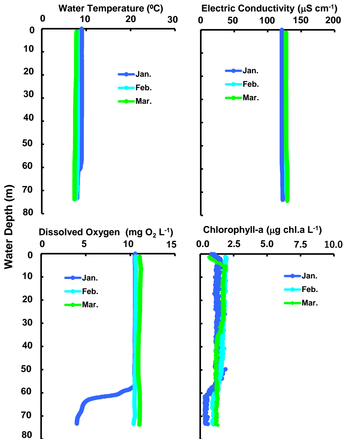
Changes of vertical distribution in water temperature, electric conductivity, dissolved oxygen concn., chlorophyll-a amount at Stn.le-1 in the north basin of Lake Biwa from January to March 2023.
