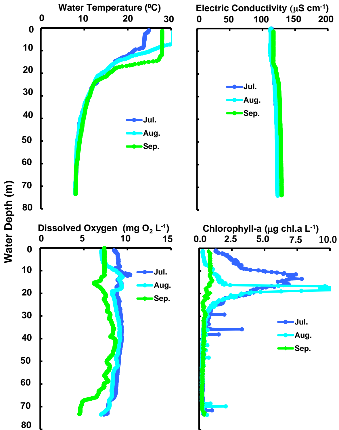
Changes of vertical distribution in water temperature, conductivity, dissolved oxygen concn., chlorophyll-a amount at Stn.le-1 in the north basin of Lake Biwa from July to September 2023.
