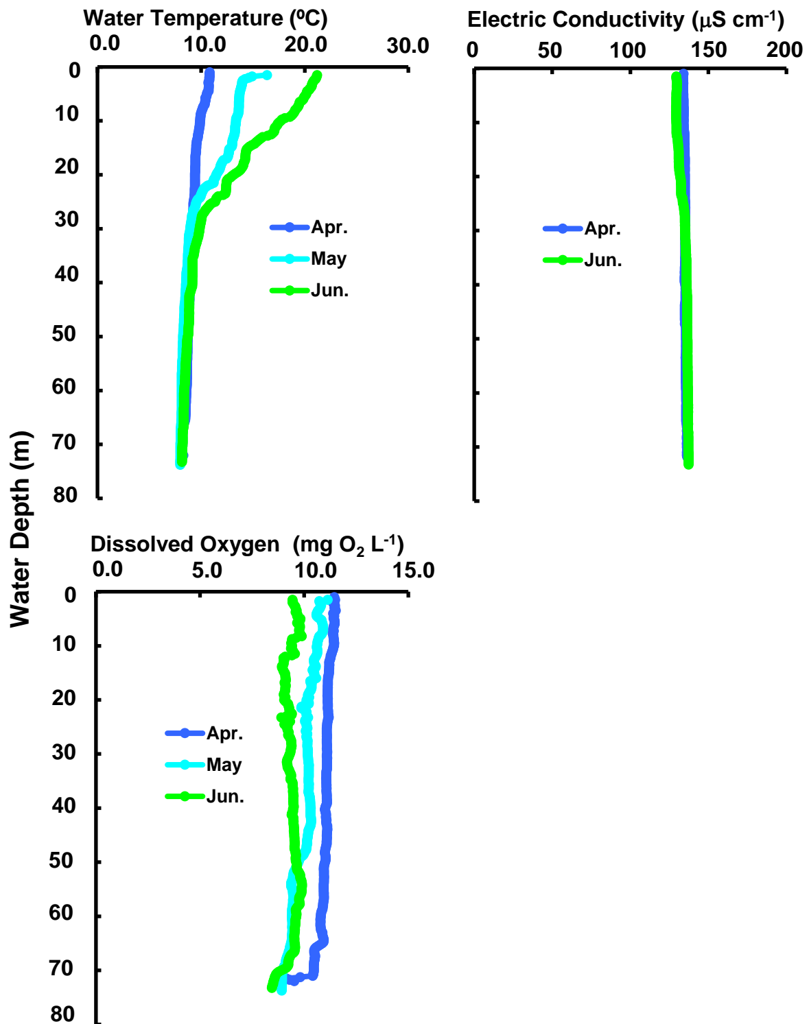
Changes of vertical distribution in water temperature, electric conductivity, dissolved oxygen concn. at Stn.le-1 in the north basin of Lake Biwa from April to June 2010.
