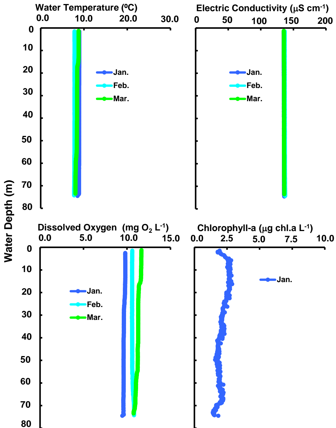
Changes of vertical distribution in water temperature, electric conductivity, dissolved oxygen concn., chlorophyll-a amount at Stn.le-1 in the north basin of Lake Biwa from January to March 2010.
