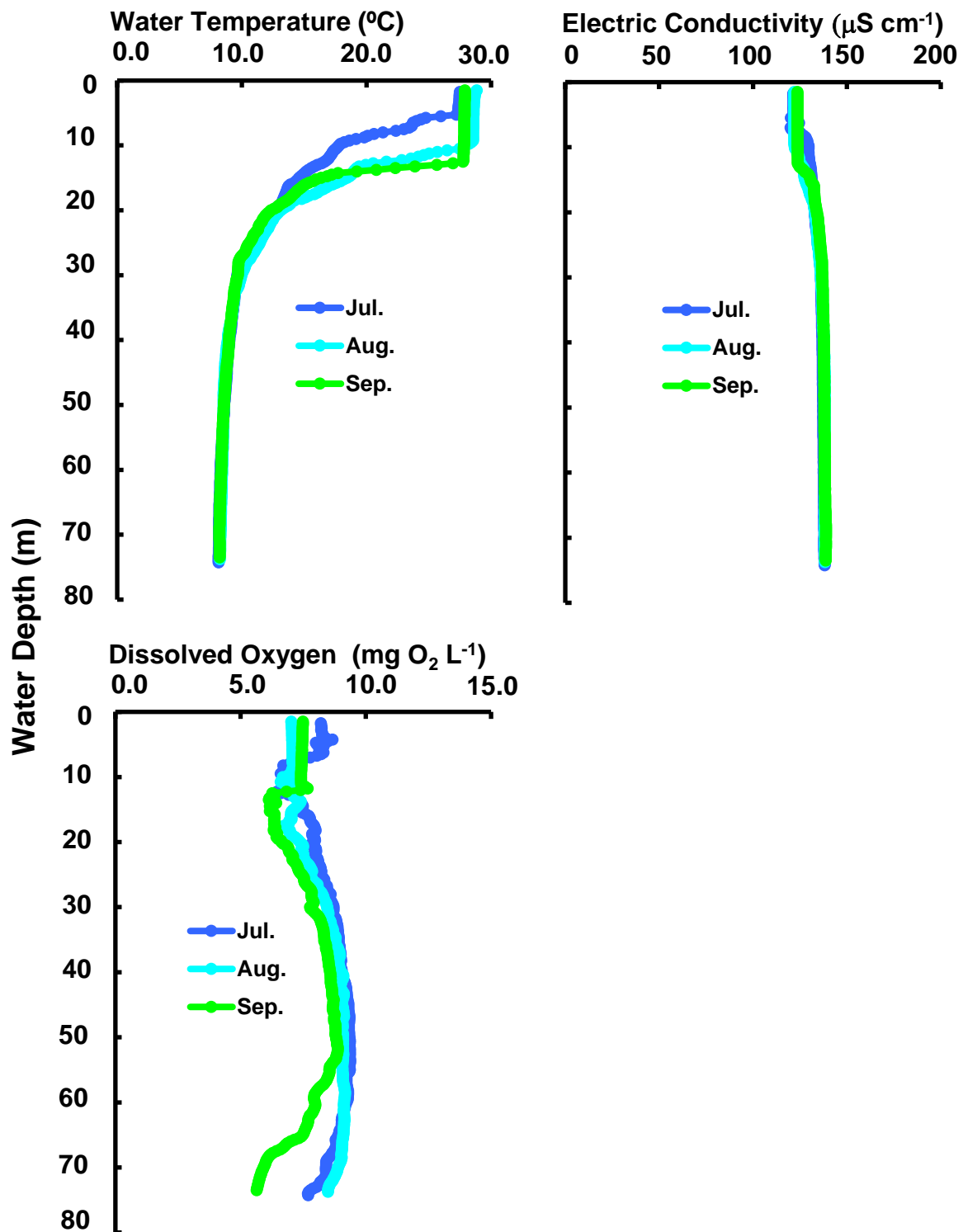
Changes of vertical distribution in water temperature, conductivity, dissolved oxygen concn. at Stn.le-1 in the north basin of Lake Biwa from July to September 2010.
