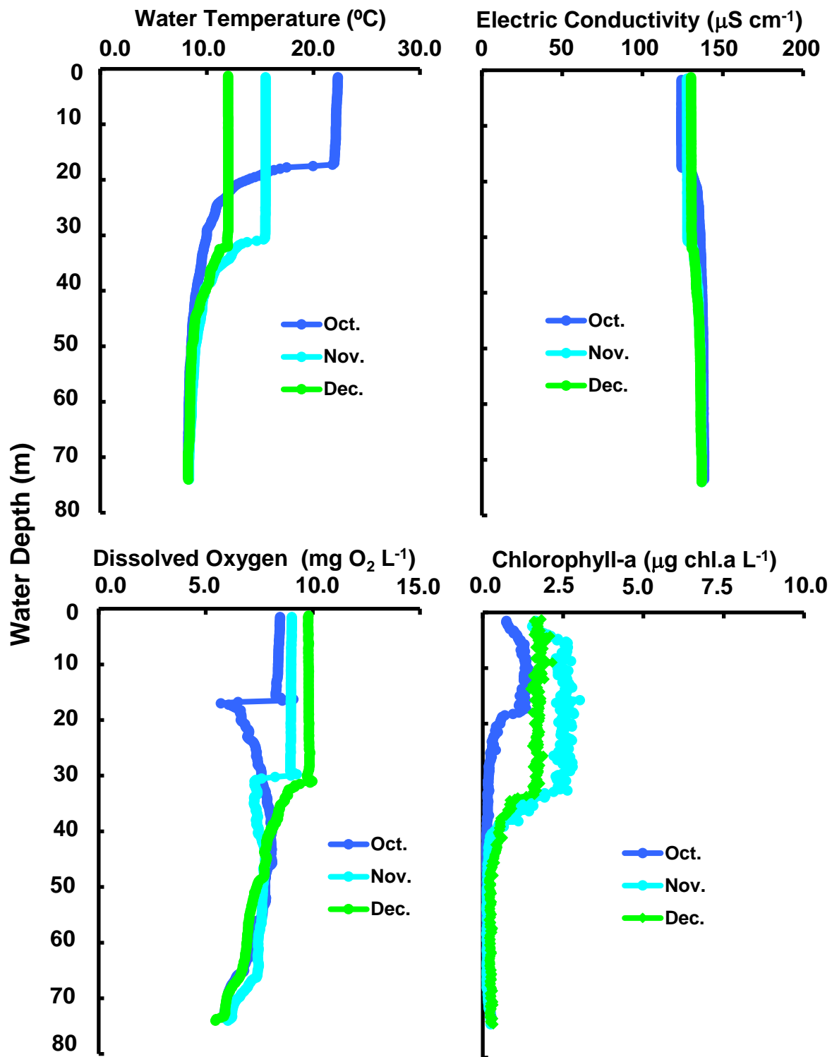
Changes of vertical distribution in water temperature, electric conductivity, dissolved oxygen concn., chlorophyll-a amount at Stn.le-1 in the north basin of Lake Biwa from October to December 2010.
