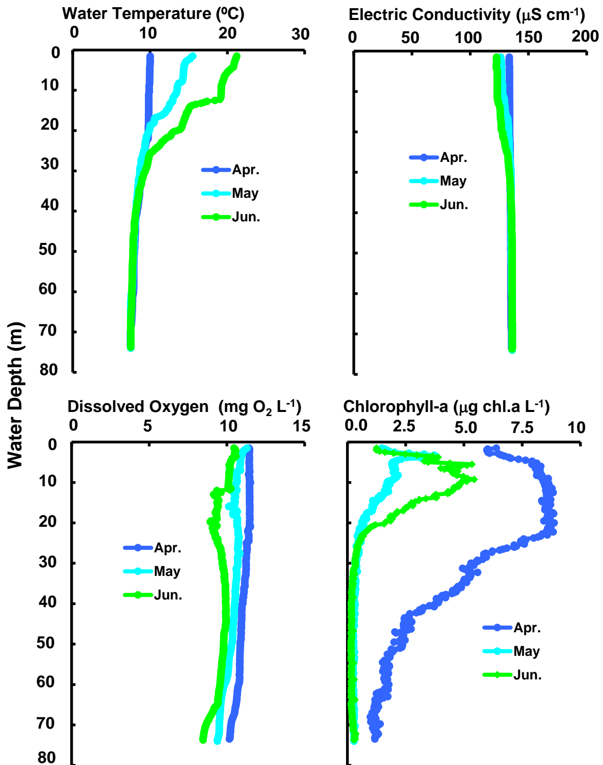
Changes of vertical distribution in water temperature, electric conductivity, dissolved oxygen concn., chlorophyll-a amount at Stn.le-1 in the north basin of Lake Biwa from April to June 2011.
