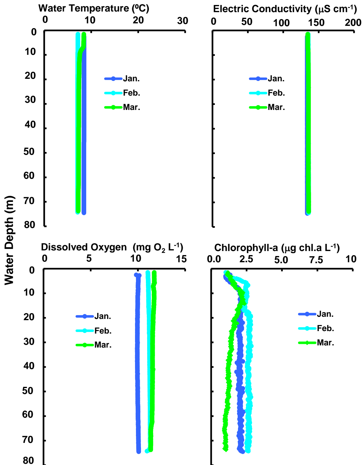
Changes of vertical distribution in water temperature, electric conductivity, dissolved oxygen concn., chlorophyll-a amount at Stn.le-1 in the north basin of Lake Biwa from January to March 2011.
