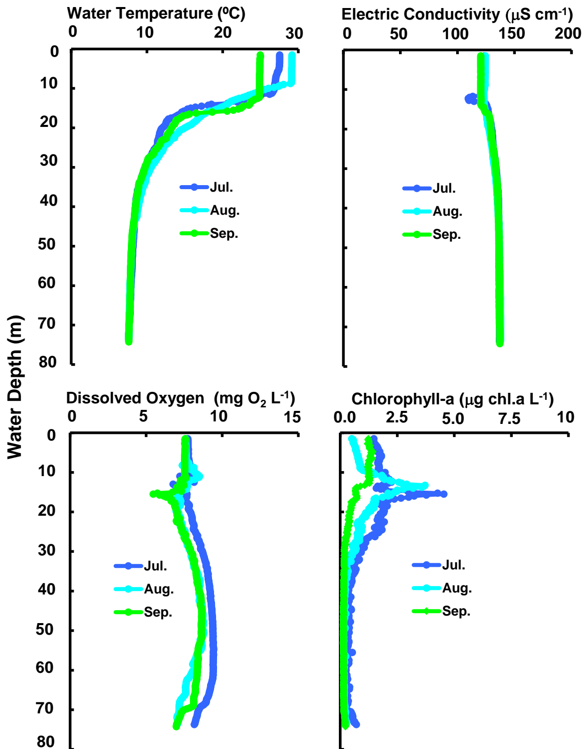
Changes of vertical distribution in water temperature, conductivity, dissolved oxygen concn., chlorophyll-a amount at Stn.le-1 in the north basin of Lake Biwa from July to September 2011.
