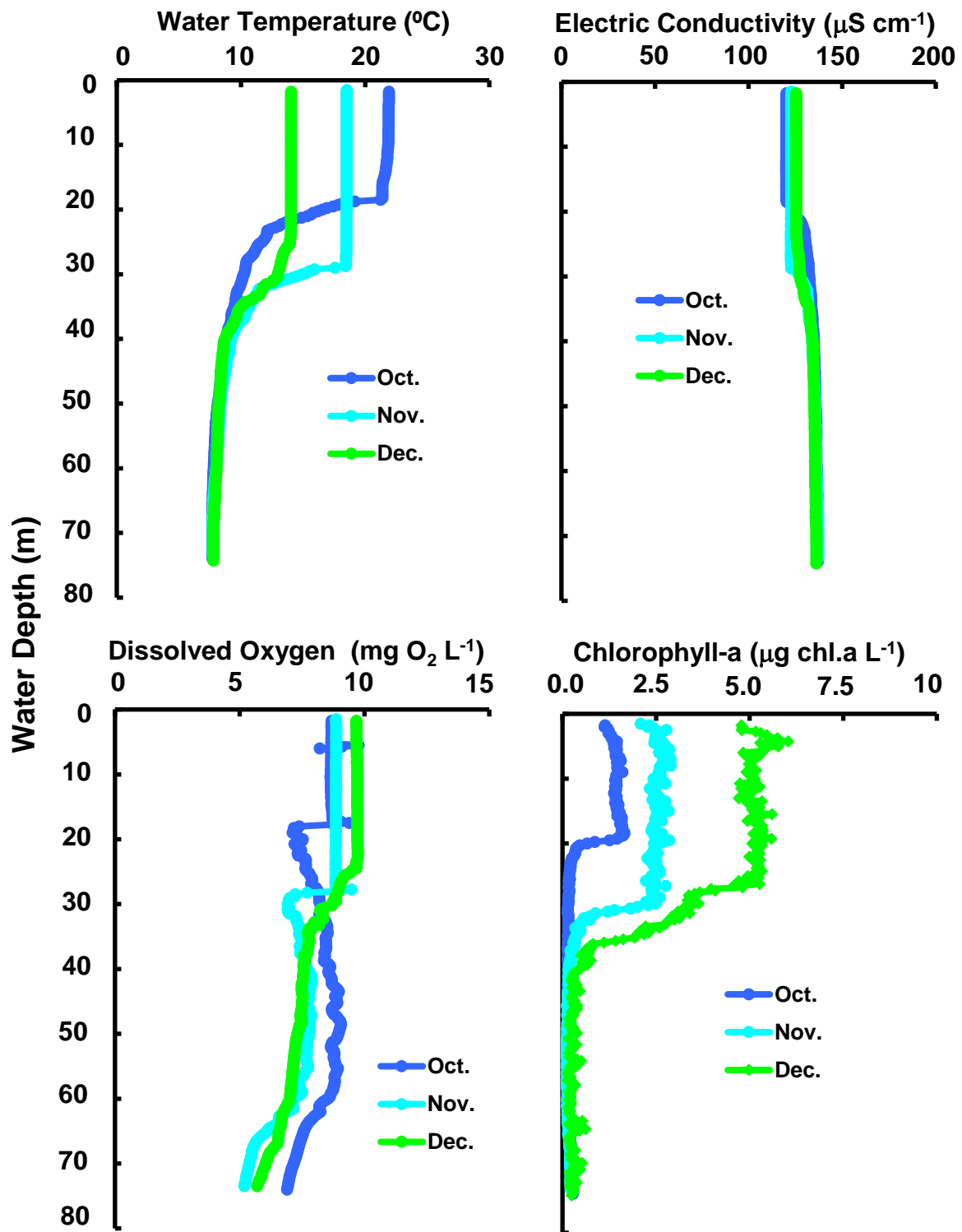
Changes of vertical distribution in water temperature, electric conductivity, dissolved oxygen concn., chlorophyll-a amount at Stn.le-1 in the north basin of Lake Biwa from October to December 2011.
