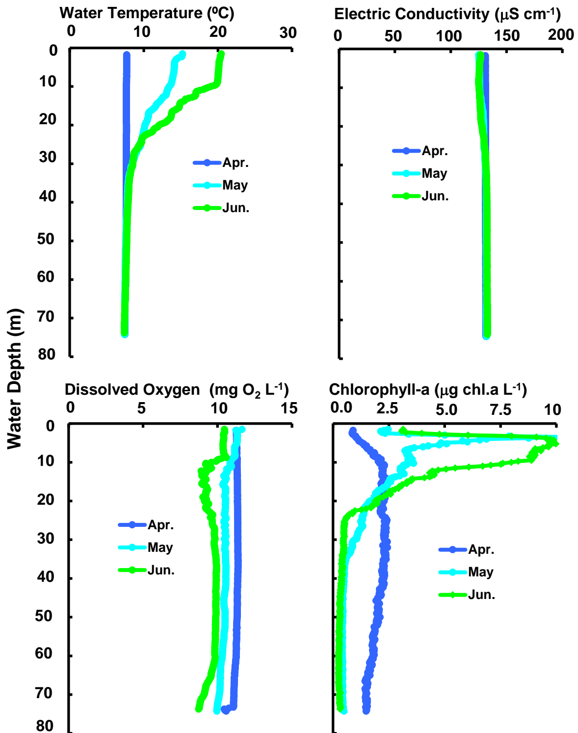
Changes of vertical distribution in water temperature, electric conductivity, dissolved oxygen concn., chlorophyll-a amount at Stn.le-1 in the north basin of Lake Biwa from April to June 2012.
