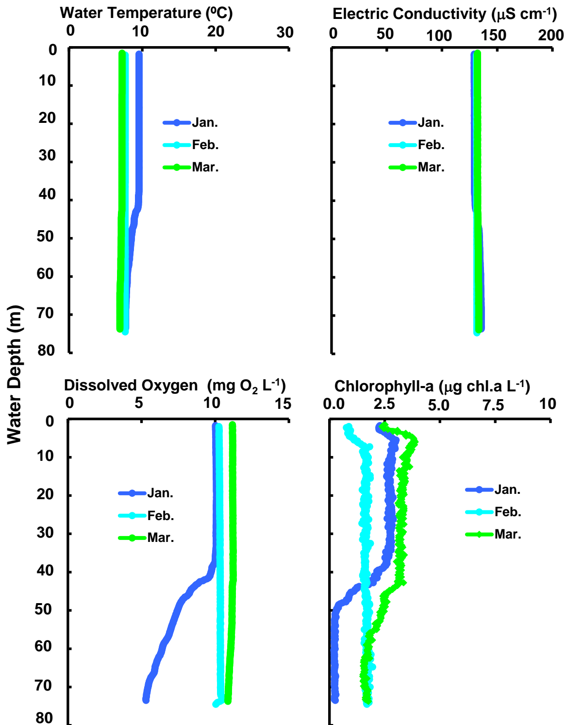
Changes of vertical distribution in water temperature, electric conductivity, dissolved oxygen concn., chlorophyll-a amount at Stn.le-1 in the north basin of Lake Biwa from January to March 2012.
