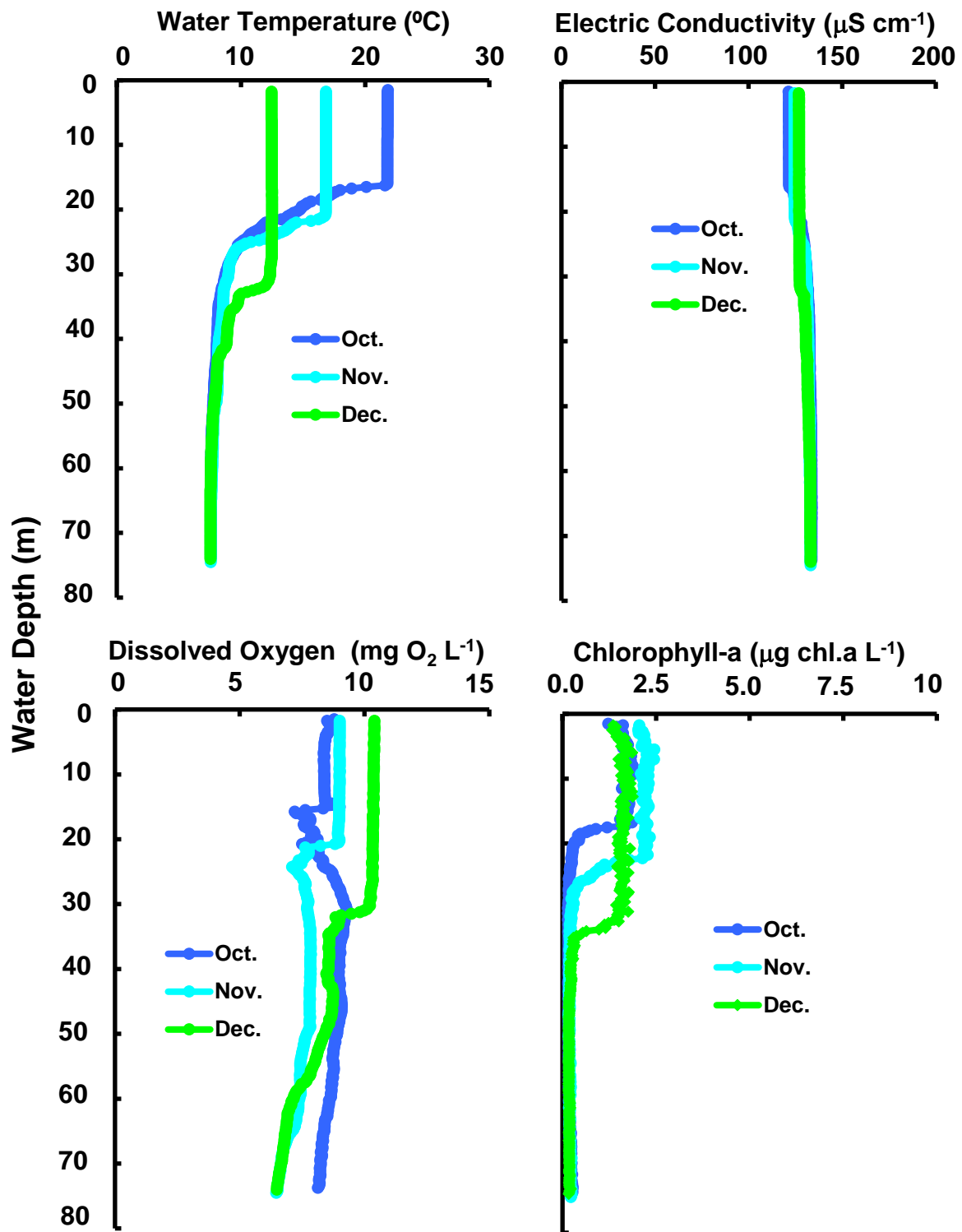
Changes of vertical distribution in water temperature, electric conductivity, dissolved oxygen concn., chlorophyll-a amount at Stn.le-1 in the north basin of Lake Biwa from October to December 2012.
