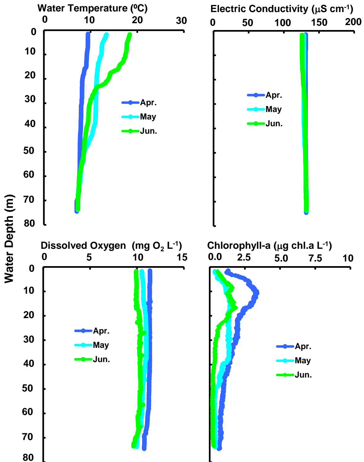
Changes of vertical distribution in water temperature, electric conductivity, dissolved oxygen concn., chlorophyll-a amount at Stn.le-1 in the north basin of Lake Biwa from April to June 2013.
