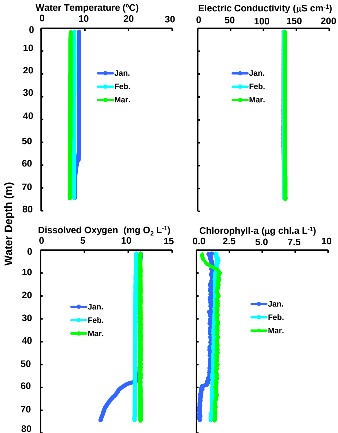
Changes of vertical distribution in water temperature, electric conductivity, dissolved oxygen concn., chlorophyll-a amount at Stn.le-1 in the north basin of Lake Biwa from January to March 2013.
