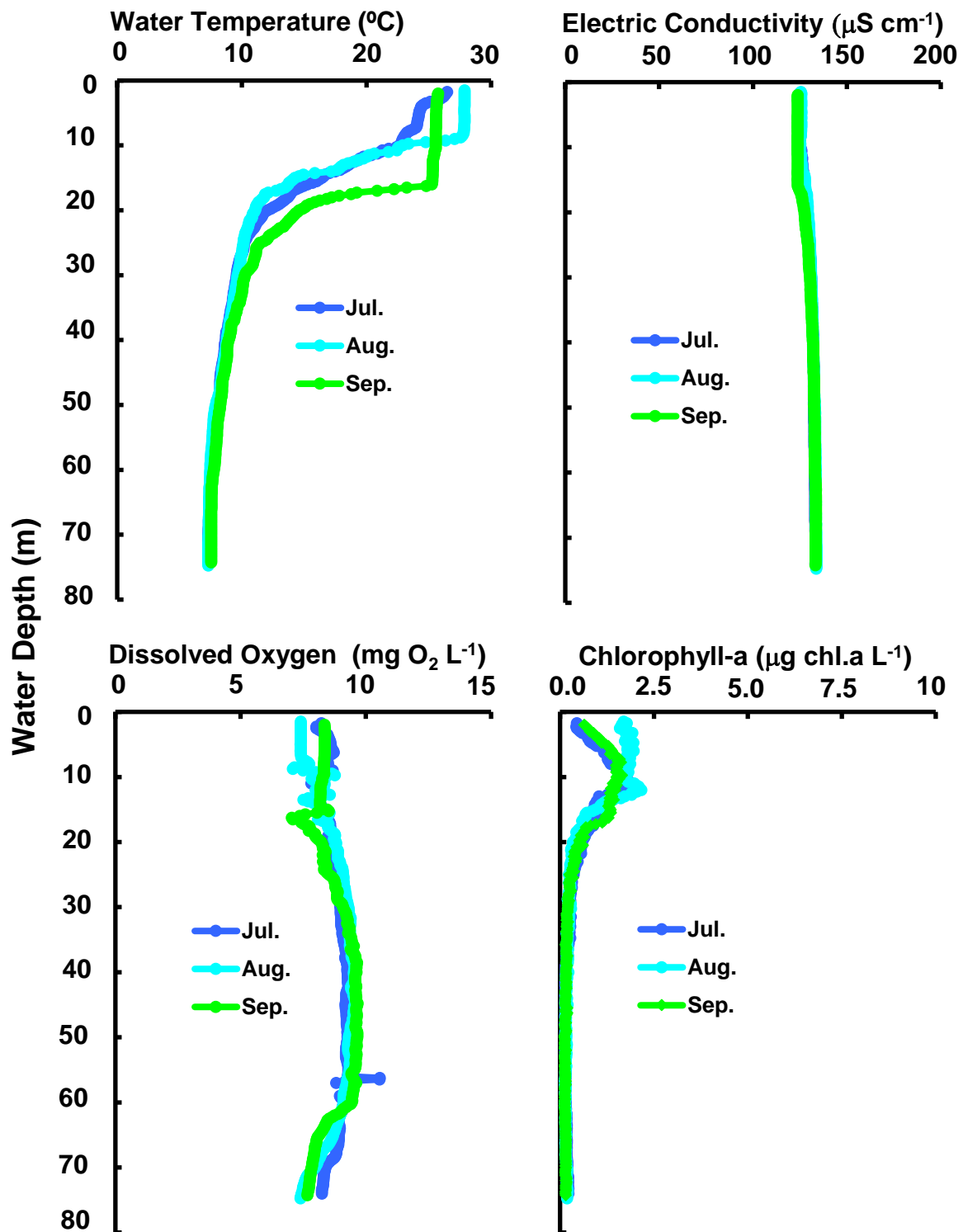
Changes of vertical distribution in water temperature, conductivity, dissolved oxygen concn., chlorophyll-a amount at Stn.le-1 in the north basin of Lake Biwa from July to September 2013.
