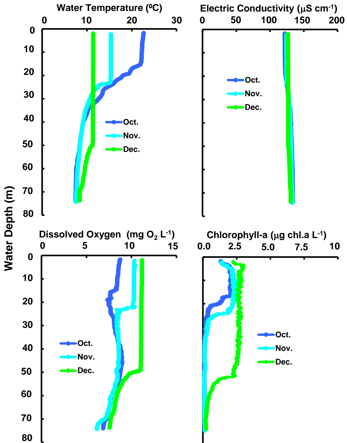
Changes of vertical distribution in water temperature, electric conductivity, dissolved oxygen concn., chlorophyll-a amount at Stn.le-1 in the north basin of Lake Biwa from October to December 2013.
