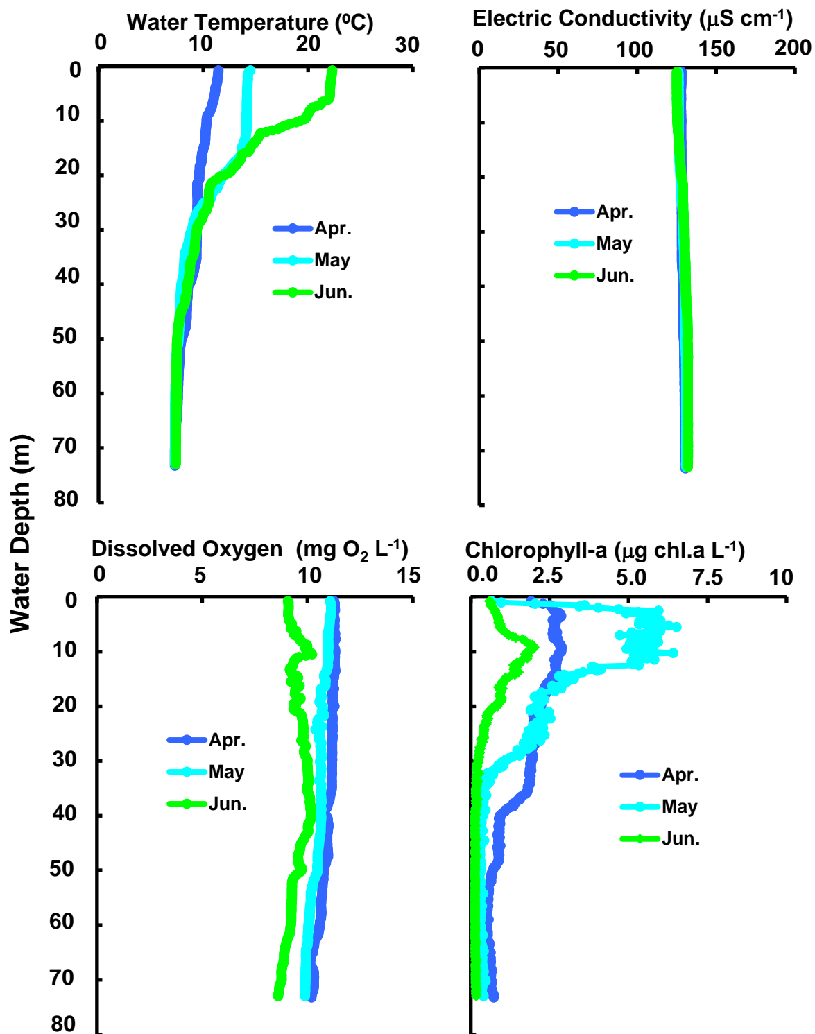
Changes of vertical distribution in water temperature, electric conductivity, dissolved oxygen concn., chlorophyll-a amount at Stn.le-1 in the north basin of Lake Biwa from April to June 2014.
