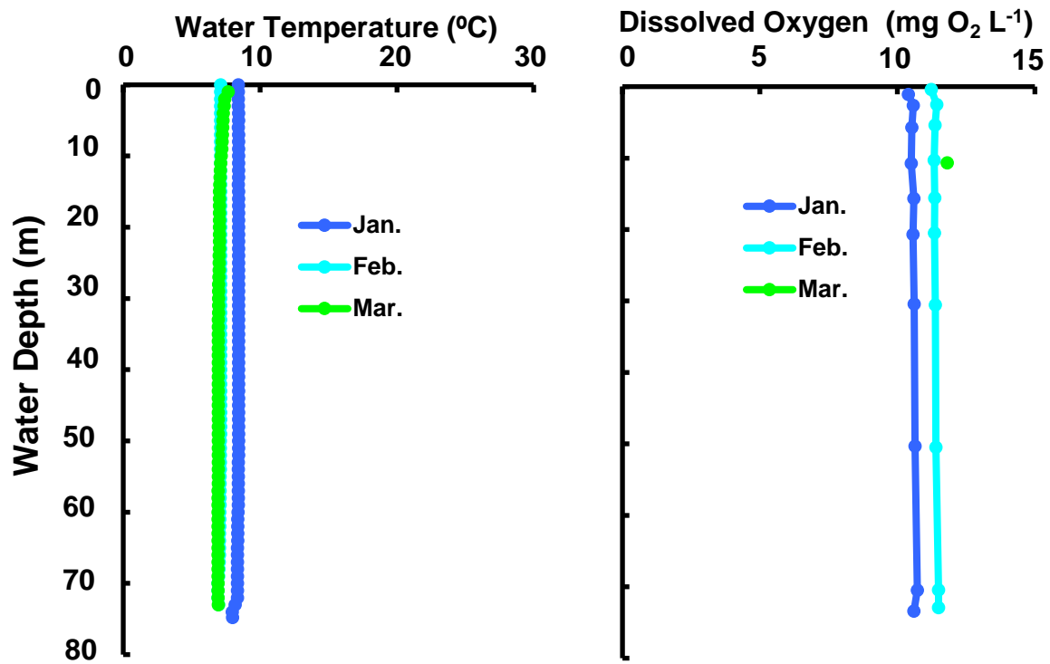
Changes of vertical distribution in water temperature, dissolved oxygen concn. at Stn.le-1 in the north basin of Lake Biwa from January to March 2014.
