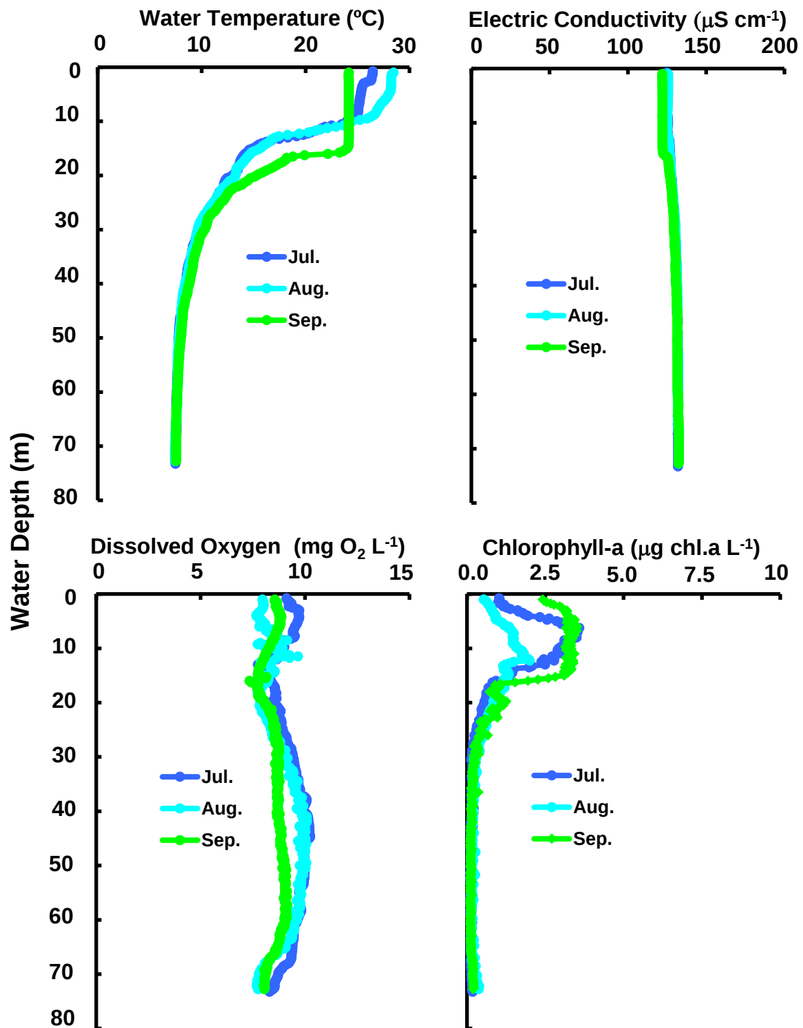
Changes of vertical distribution in water temperature, conductivity, dissolved oxygen concn., chlorophyll-a amount at Stn.le-1 in the north basin of Lake Biwa from July to September 2014.
