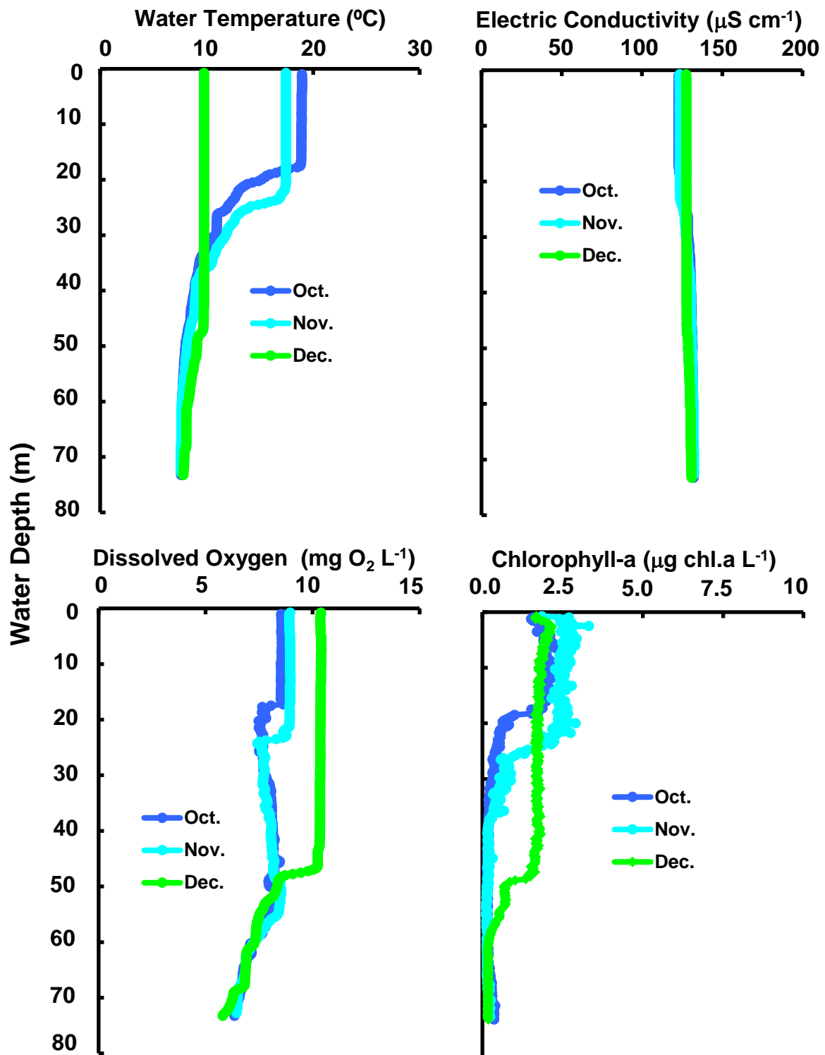
Changes of vertical distribution in water temperature, electric conductivity, dissolved oxygen concn., chlorophyll-a amount at Stn.le-1 in the north basin of Lake Biwa from October to December 2014.
