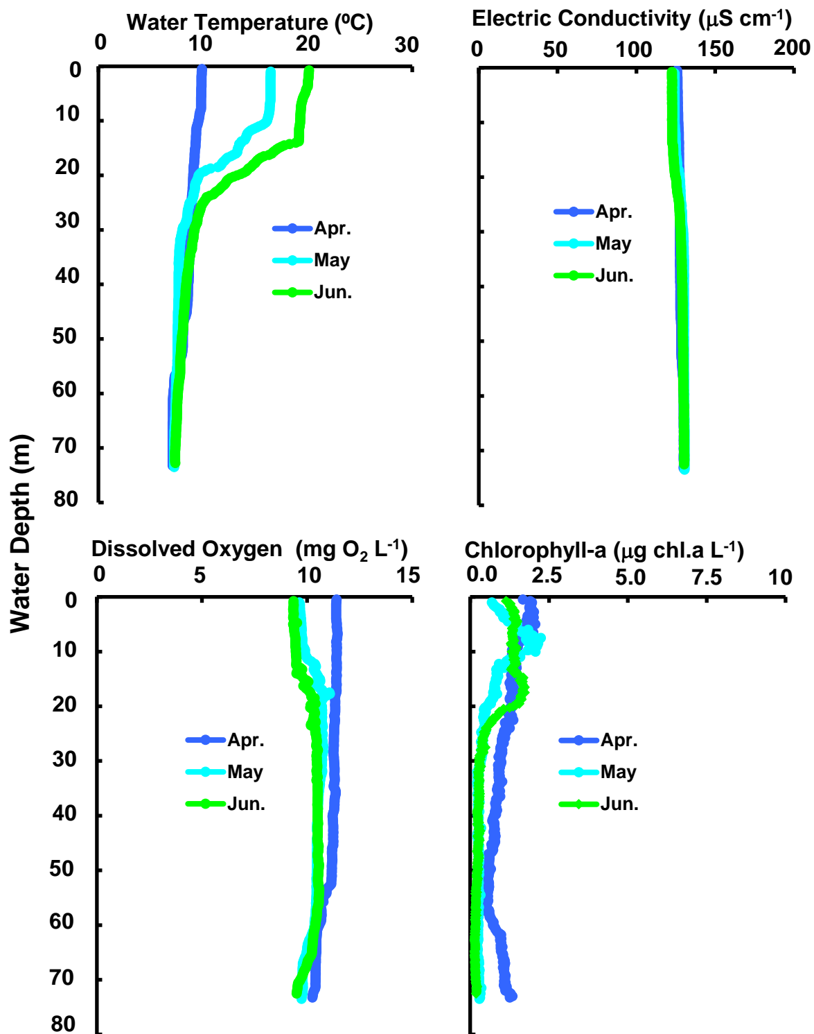
Changes of vertical distribution in water temperature, electric conductivity, dissolved oxygen concn., chlorophyll-a amount at Stn.le-1 in the north basin of Lake Biwa from April to June 2015.
