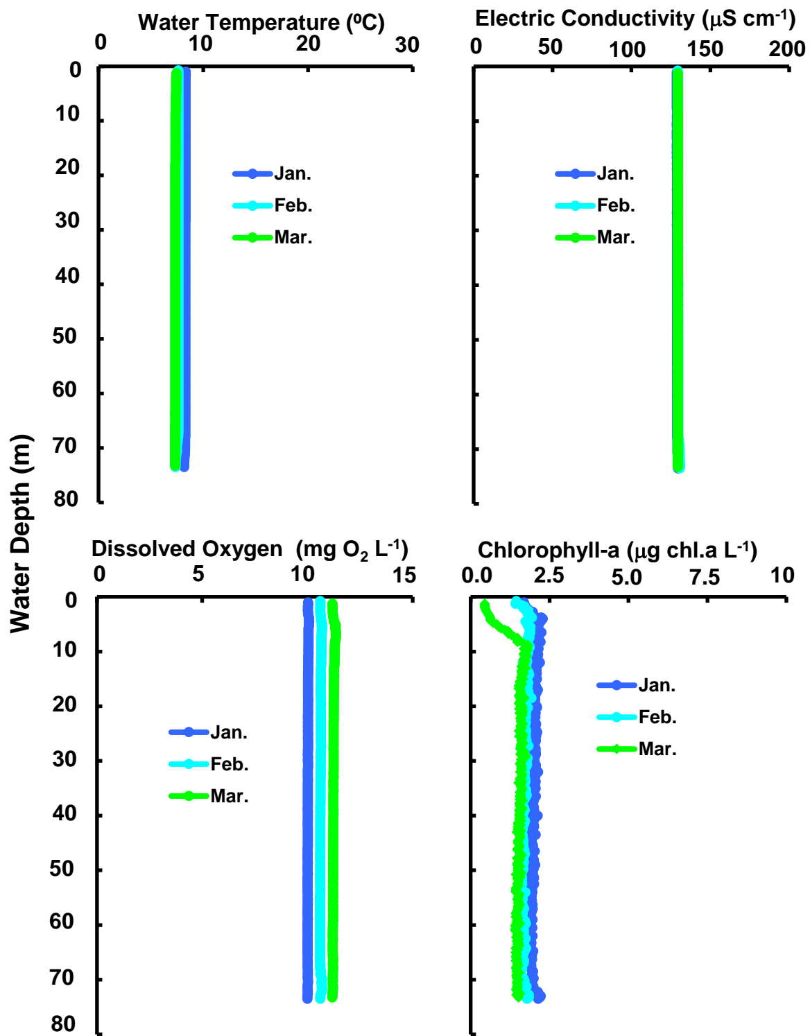
Changes of vertical distribution in water temperature, electric conductivity, dissolved oxygen concn., chlorophyll-a amount at Stn.le-1 in the north basin of Lake Biwa from January to March 2015.
