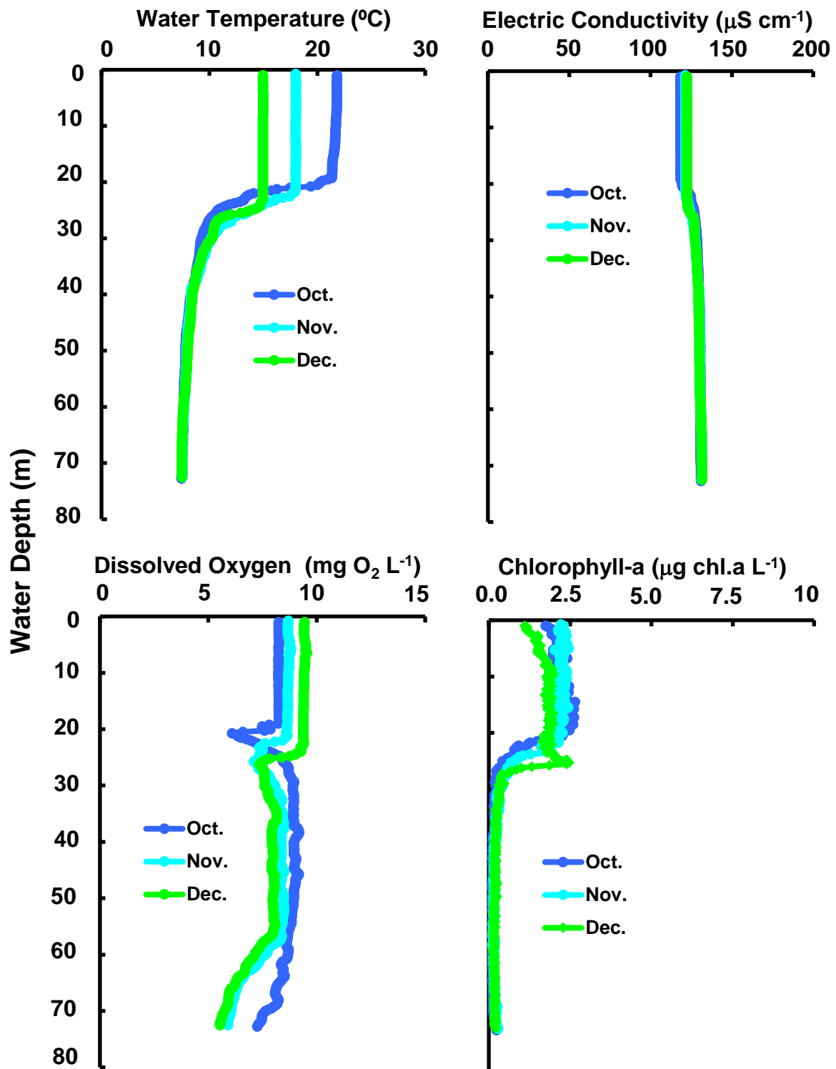
Changes of vertical distribution in water temperature, electric conductivity, dissolved oxygen concn., chlorophyll-a amount at Stn.le-1 in the north basin of Lake Biwa from October to December 2015.
