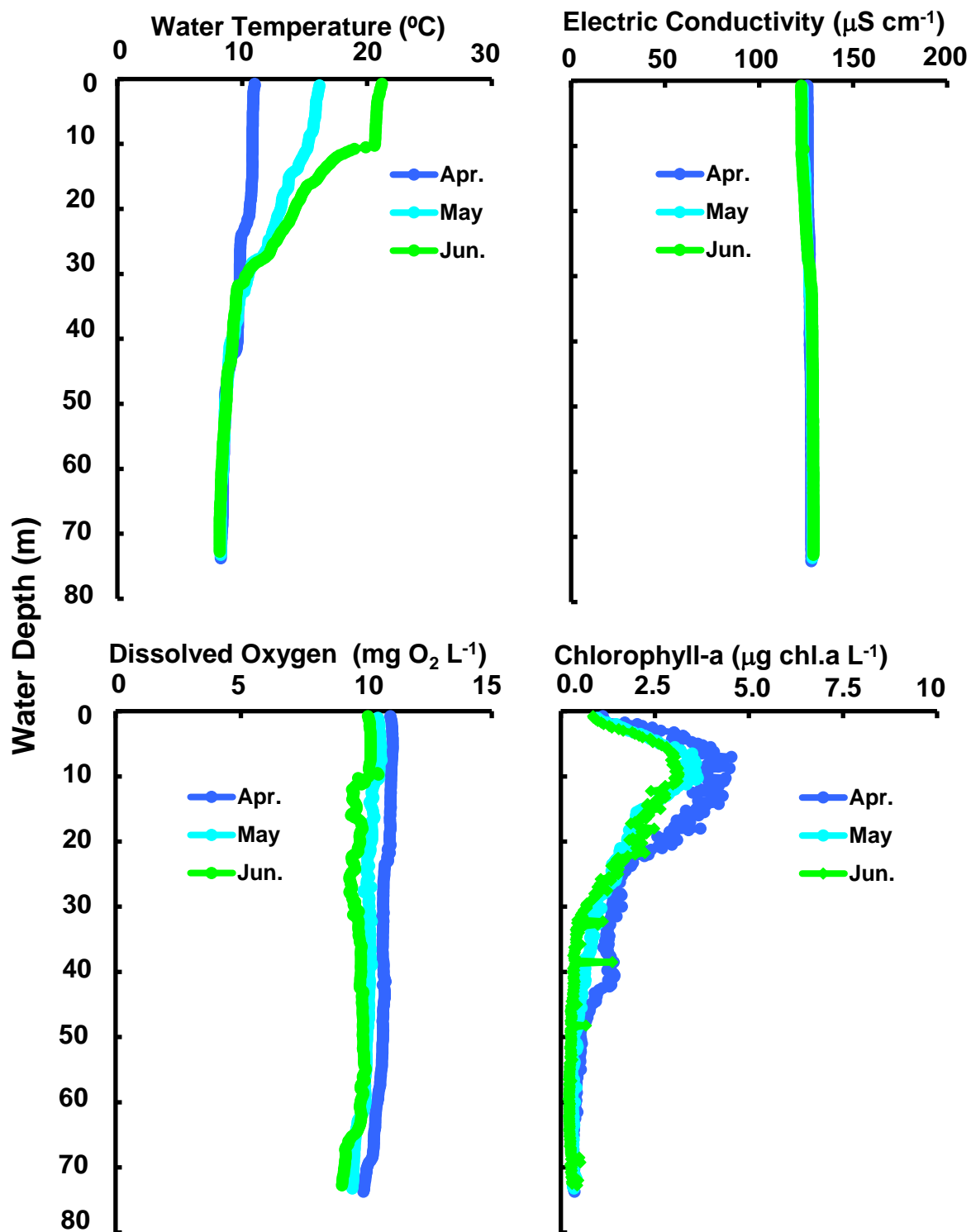
Changes of vertical distribution in water temperature, electric conductivity, dissolved oxygen concn., chlorophyll-a amount at Stn.le-1 in the north basin of Lake Biwa from April to June 2016.
