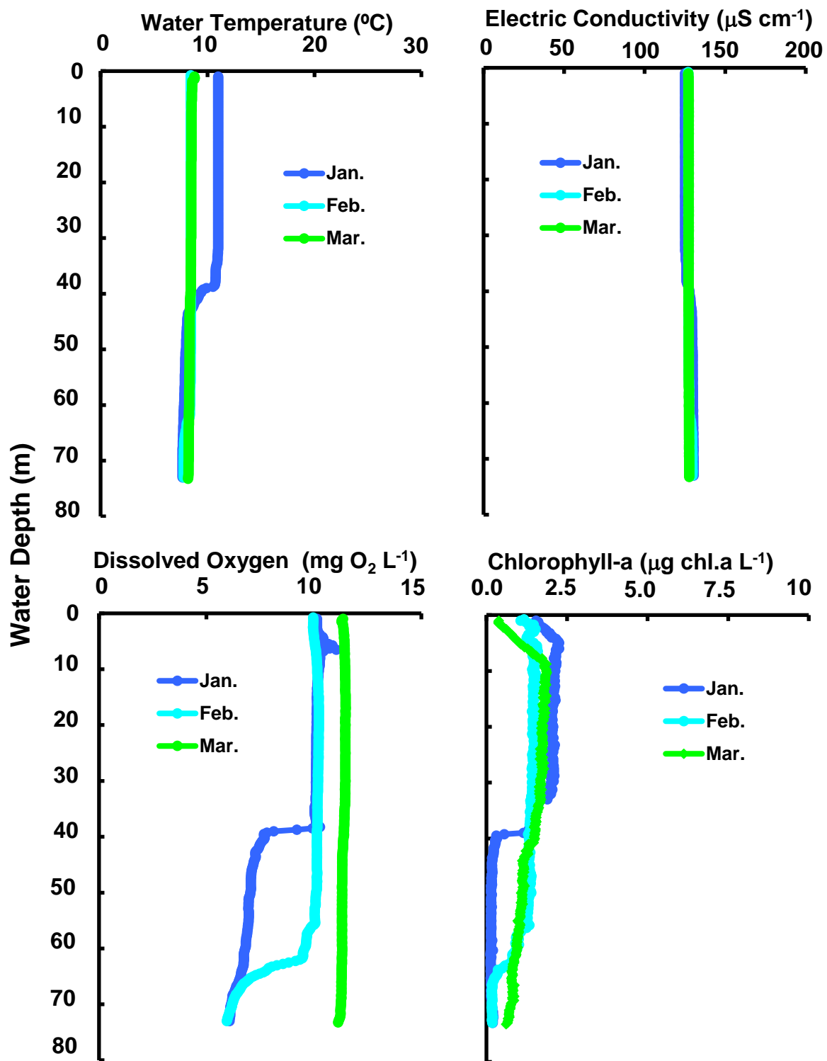
Changes of vertical distribution in water temperature, electric conductivity, dissolved oxygen concn., chlorophyll-a amount at Stn.le-1 in the north basin of Lake Biwa from January to March 2016.
