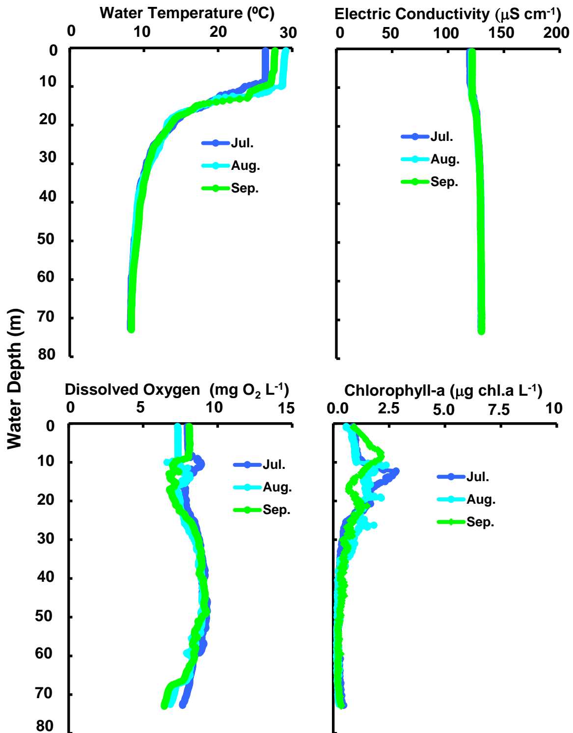
Changes of vertical distribution in water temperature, conductivity, dissolved oxygen concn., chlorophyll-a amount at Stn.le-1 in the north basin of Lake Biwa from July to September 2016.
