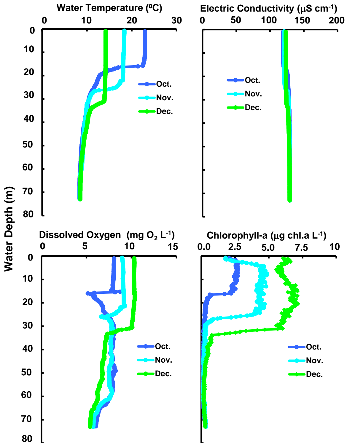
Changes of vertical distribution in water temperature, electric conductivity, dissolved oxygen concn., chlorophyll-a amount at Stn.le-1 in the north basin of Lake Biwa from October to December 2016.
