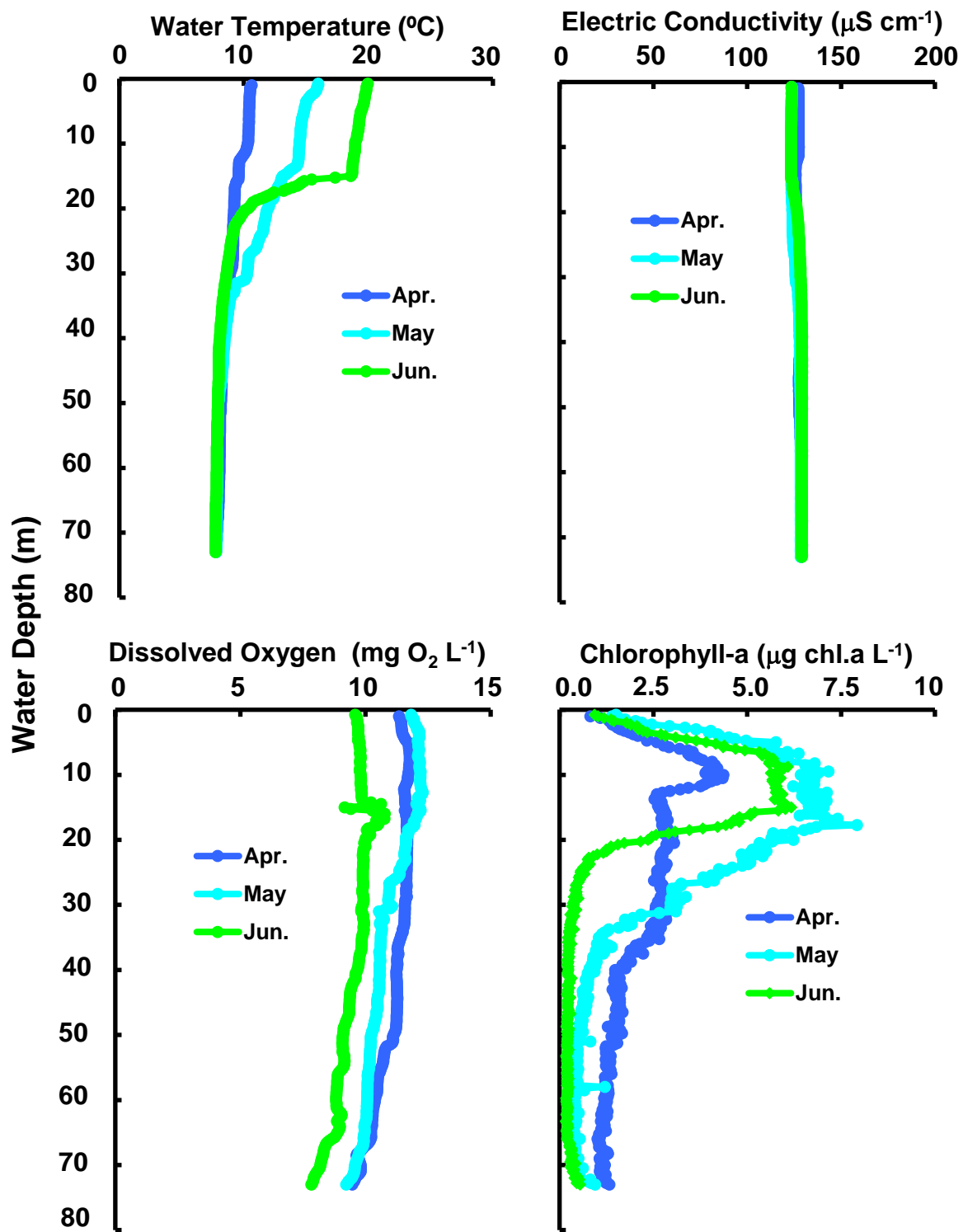
Changes of vertical distribution in water temperature, electric conductivity, dissolved oxygen concn., chlorophyll-a amount at Stn.le-1 in the north basin of Lake Biwa from April to June 2017.
