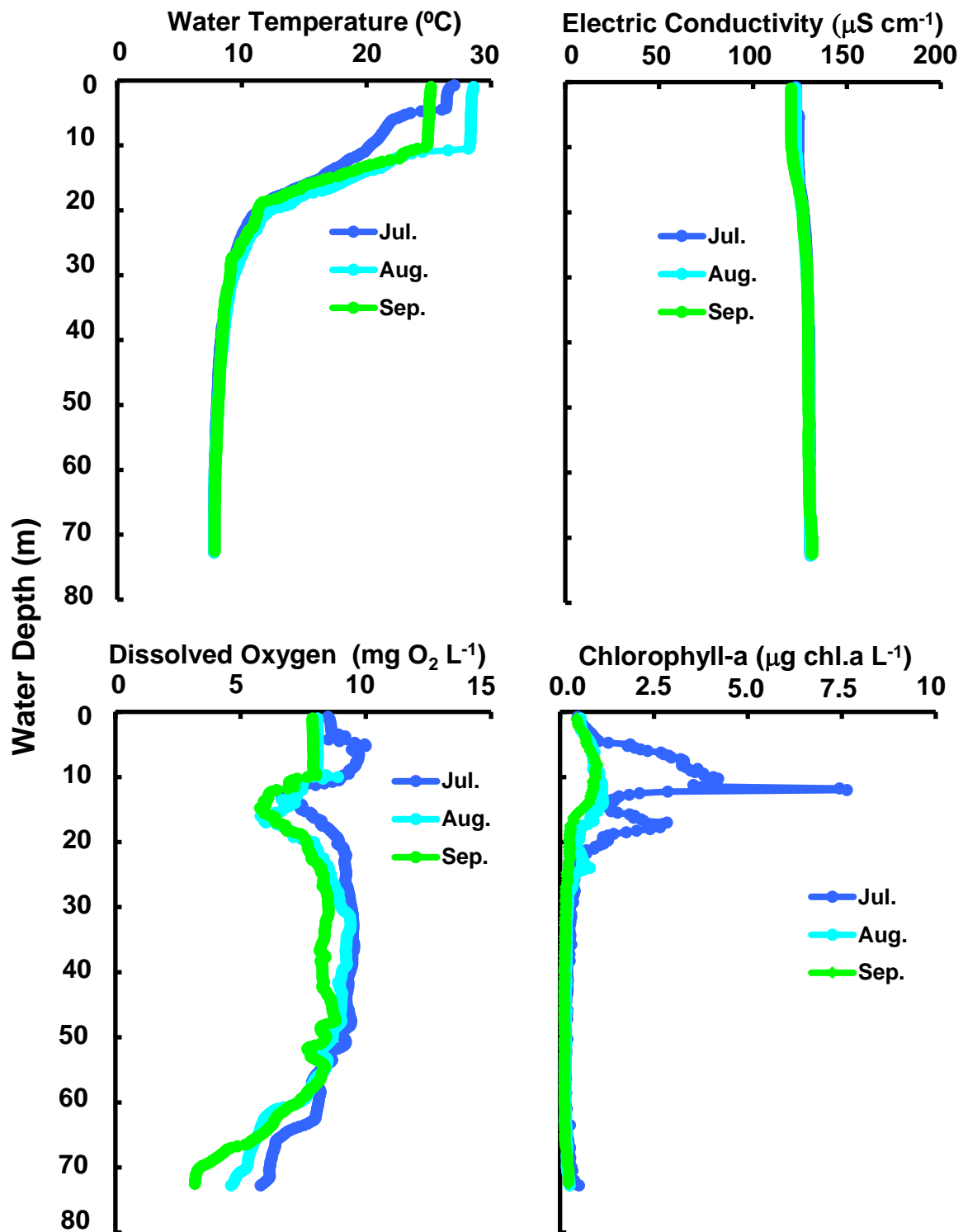
Changes of vertical distribution in water temperature, conductivity, dissolved oxygen concn., chlorophyll-a amount at Stn.le-1 in the north basin of Lake Biwa from July to September 2017.
