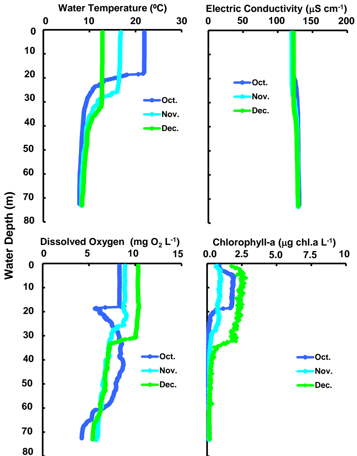
Changes of vertical distribution in water temperature, electric conductivity, dissolved oxygen concn., chlorophyll-a amount at Stn.le-1 in the north basin of Lake Biwa from October to December 2017.
