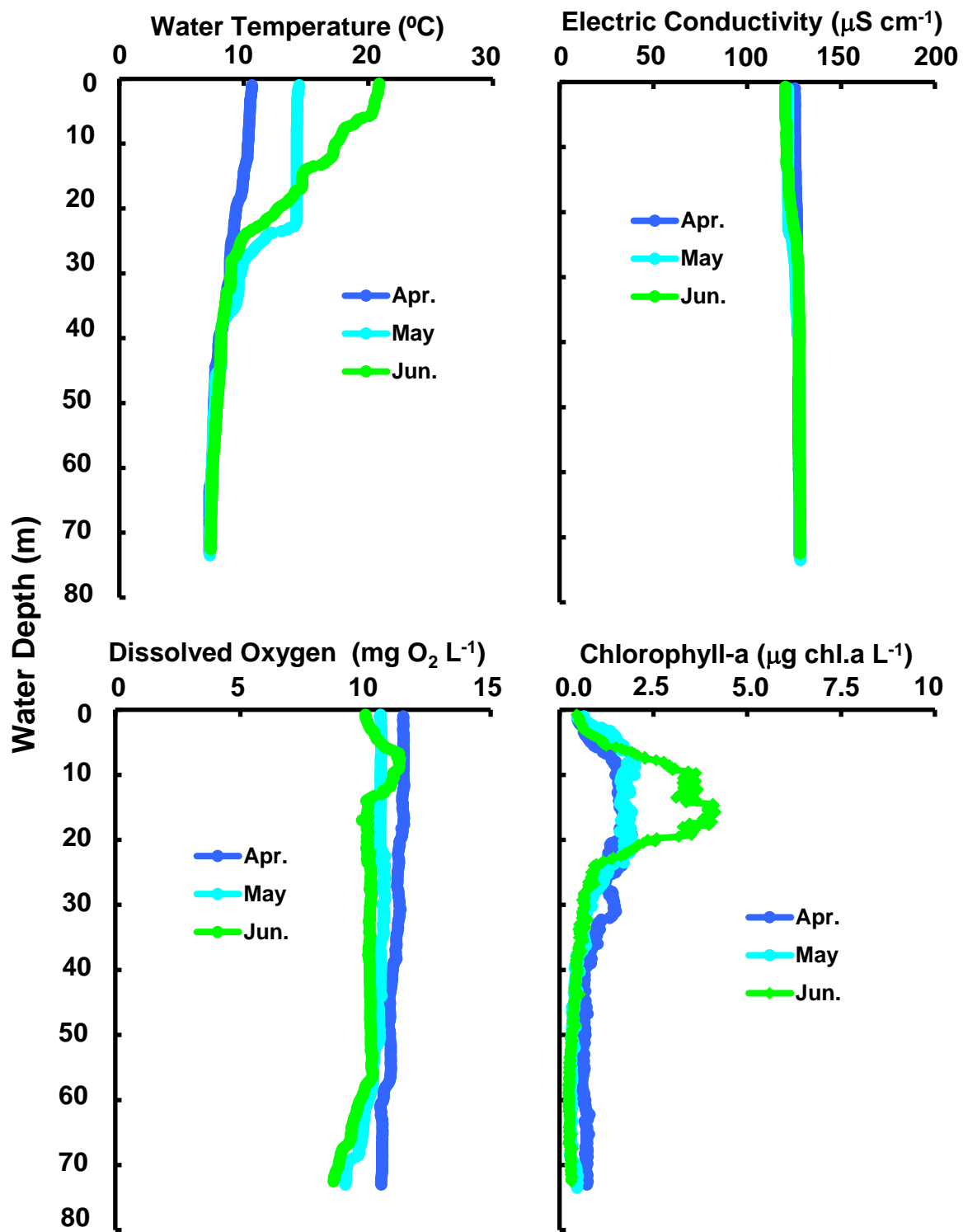
Changes of vertical distribution in water temperature, electric conductivity, dissolved oxygen concn., chlorophyll-a amount at Stn.le-1 in the north basin of Lake Biwa from April to June 2018.
