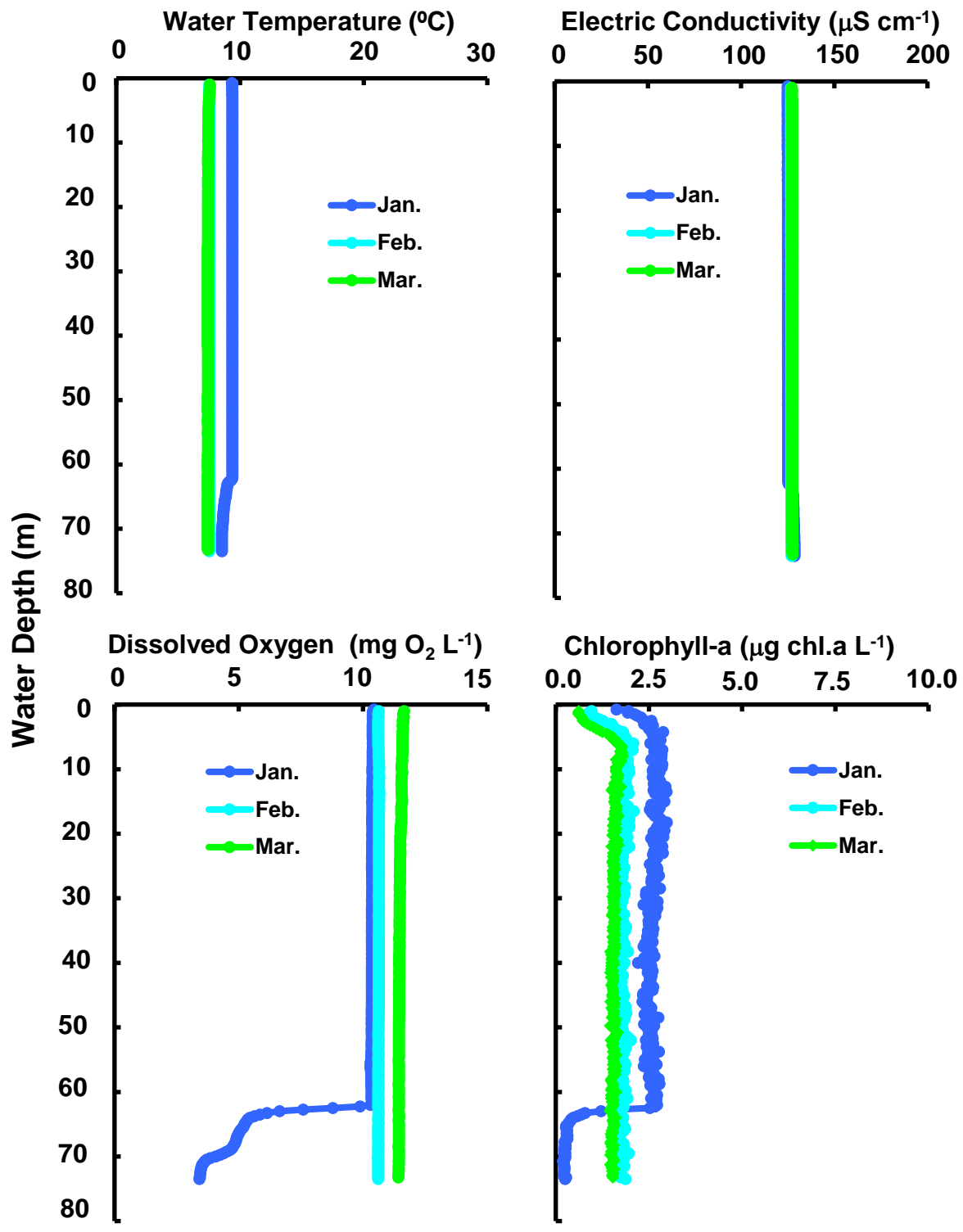
Changes of vertical distribution in water temperature, electric conductivity, dissolved oxygen concn., chlorophyll-a amount at Stn.le-1 in the north basin of Lake Biwa from January to March 2018.
