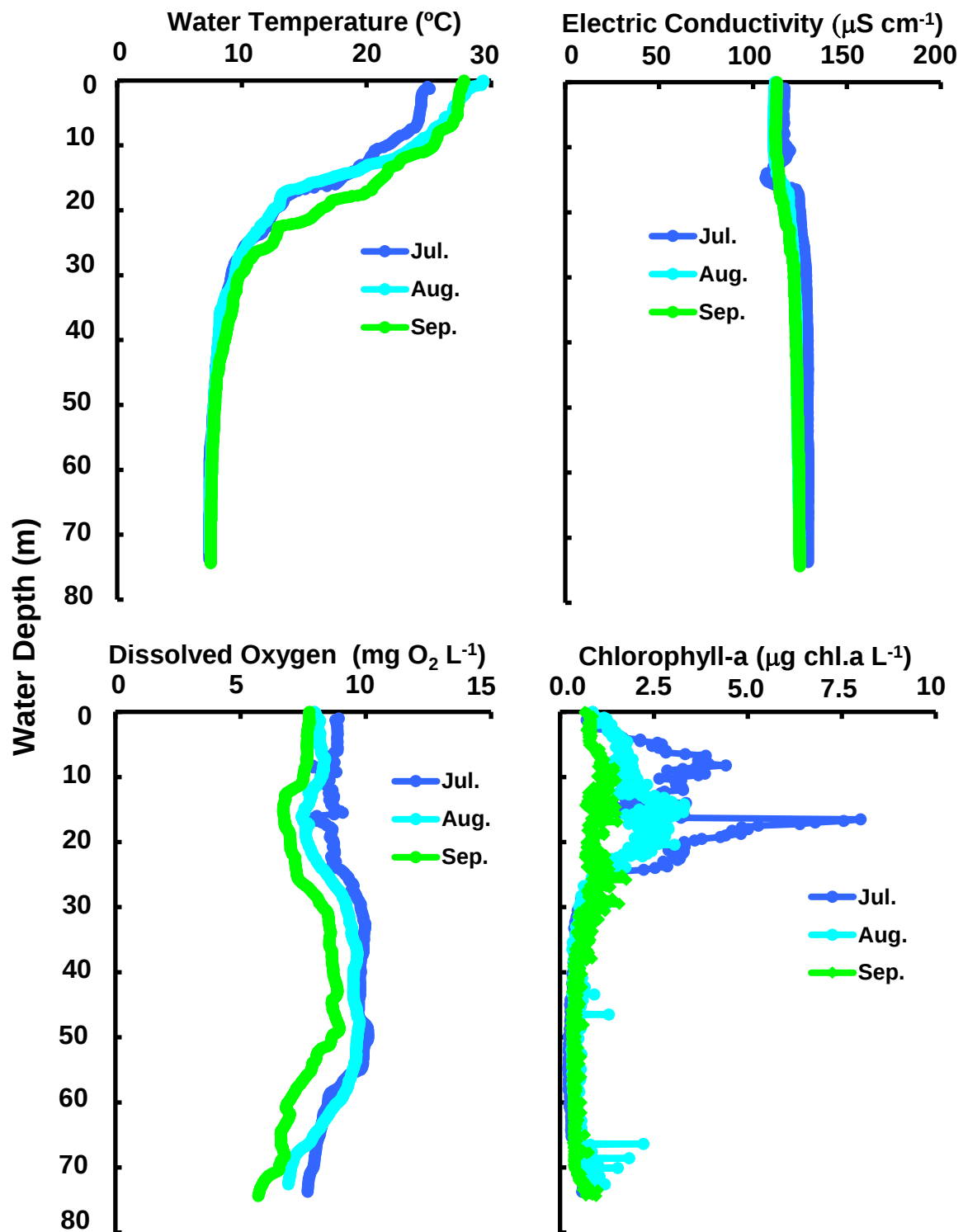
Changes of vertical distribution in water temperature, conductivity, dissolved oxygen concn., chlorophyll-a amount at Stn.le-1 in the north basin of Lake Biwa from July to September 2018.
