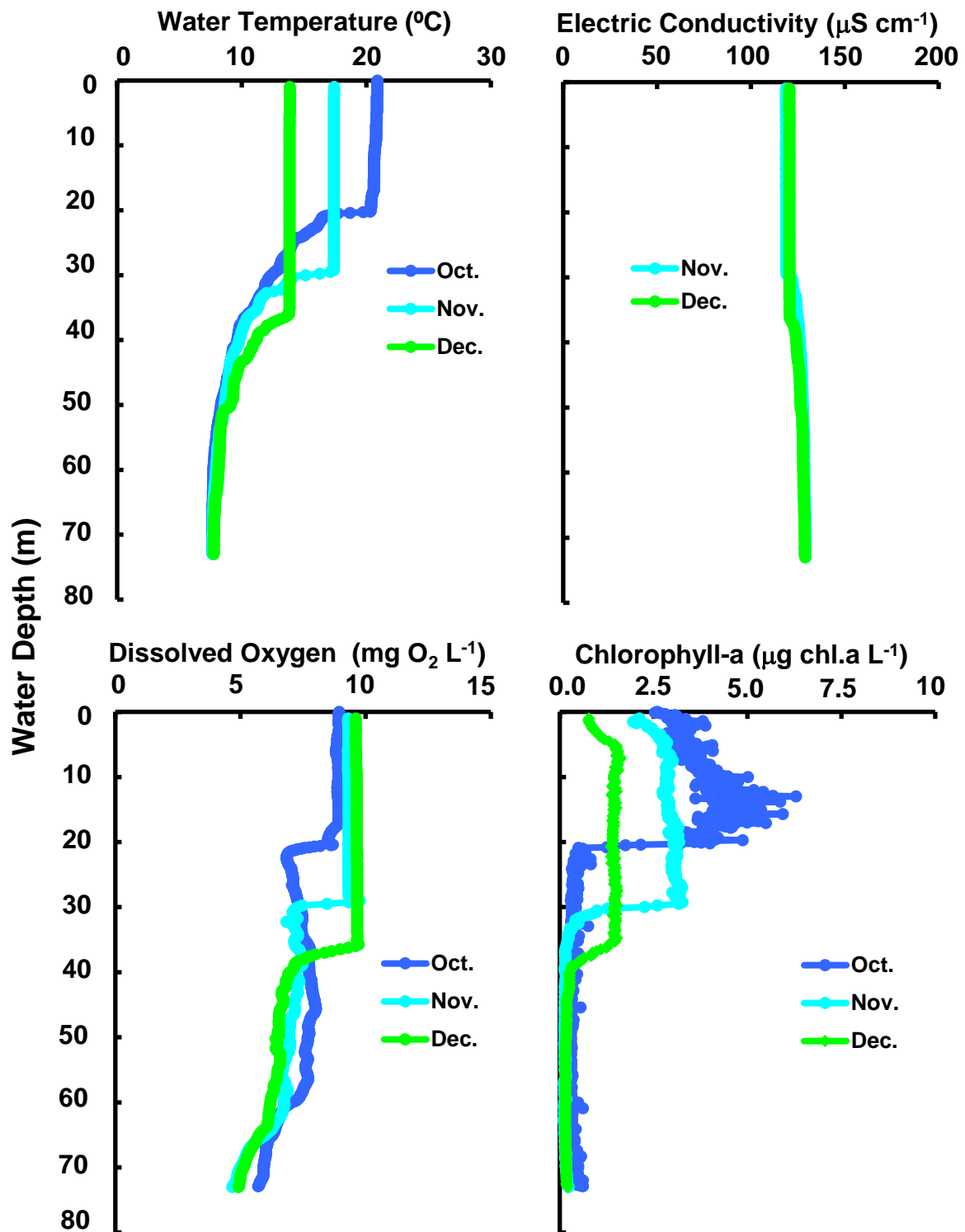
Changes of vertical distribution in water temperature, electric conductivity, dissolved oxygen concn., chlorophyll-a amount at Stn.le-1 in the north basin of Lake Biwa from October to December 2018.
