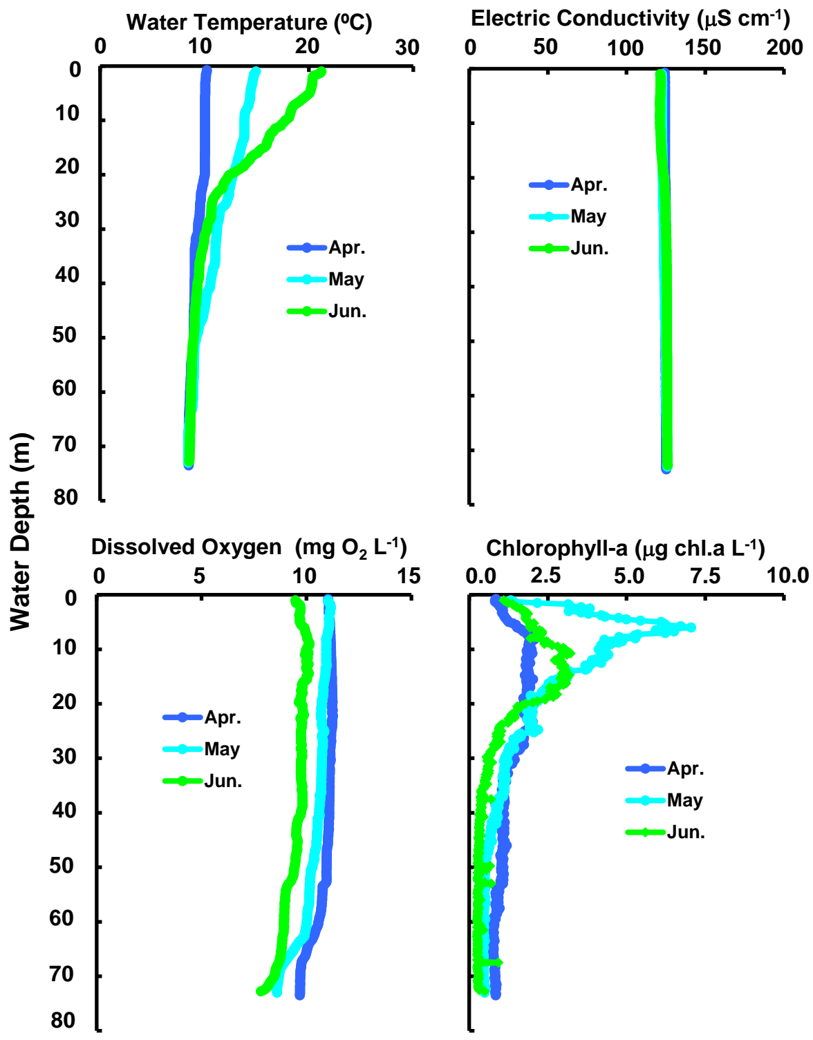
Changes of vertical distribution in water temperature, electric conductivity, dissolved oxygen concn., chlorophyll-a amount at Stn.1e-1 in the north basin of Lake Biwa from April to June 2019.
