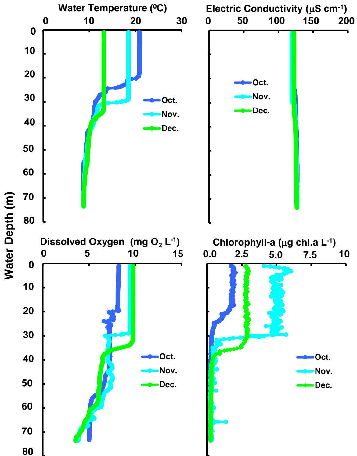
Changes of vertical distribution in water temperature, electric conductivity, dissolved oxygen concn., chlorophyll-a amount at Stn.le-1 in the north basin of Lake Biwa from October to December 2019.
