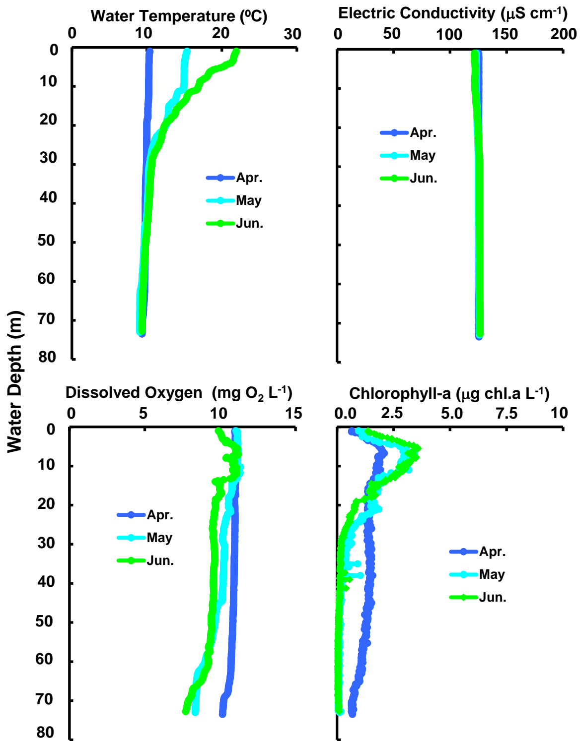
Changes of vertical distribution in water temperature, electric conductivity, dissolved oxygen concn., chlorophyll-a amount at Stn.1e-1 in the north basin of Lake Biwa from April to June 2020.
