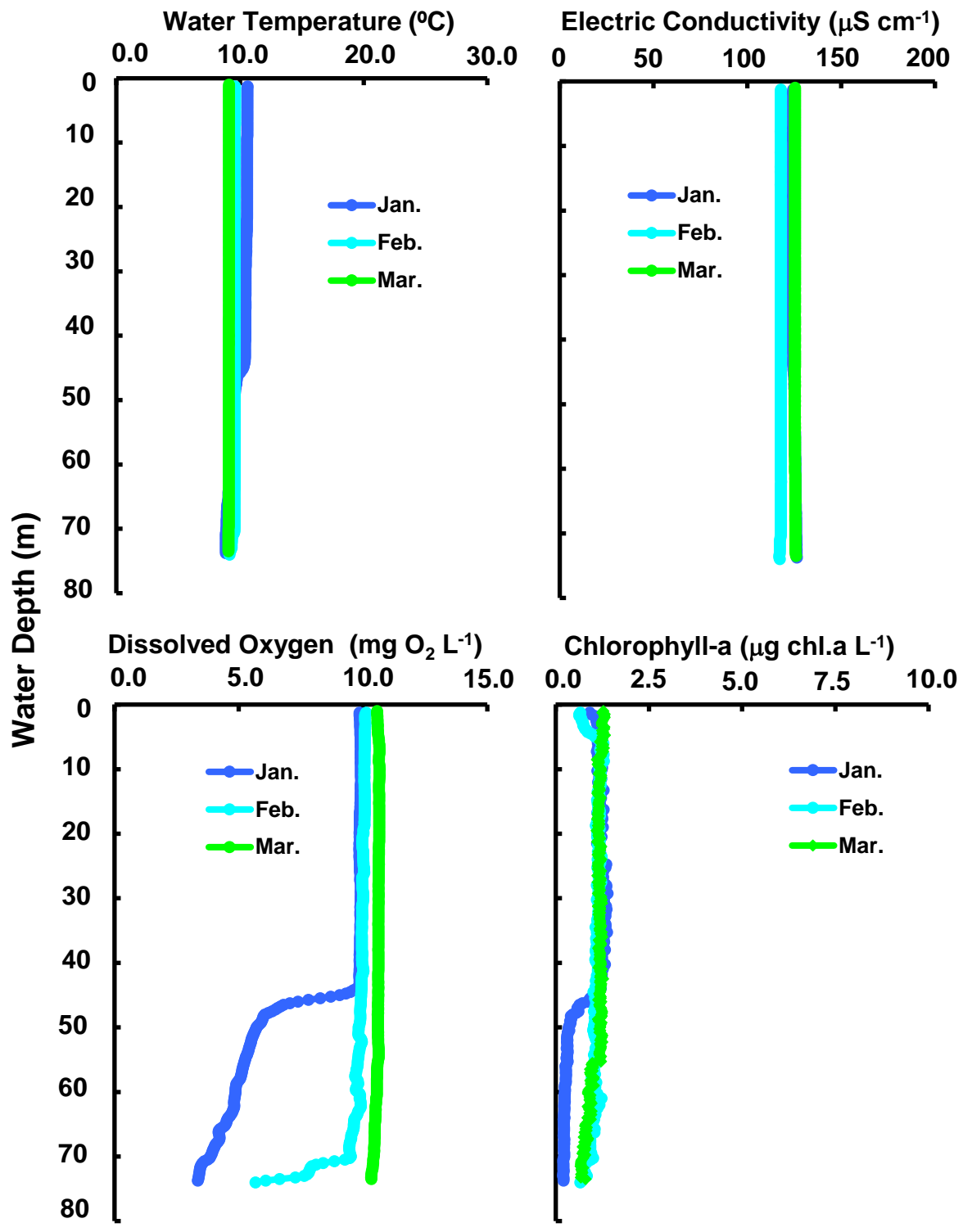
Changes of vertical distribution in water temperature, electric conductivity, dissolved oxygen concn., chlorophyll-a amount at Stn.le-1 in the north basin of Lake Biwa from January to March 2020.
