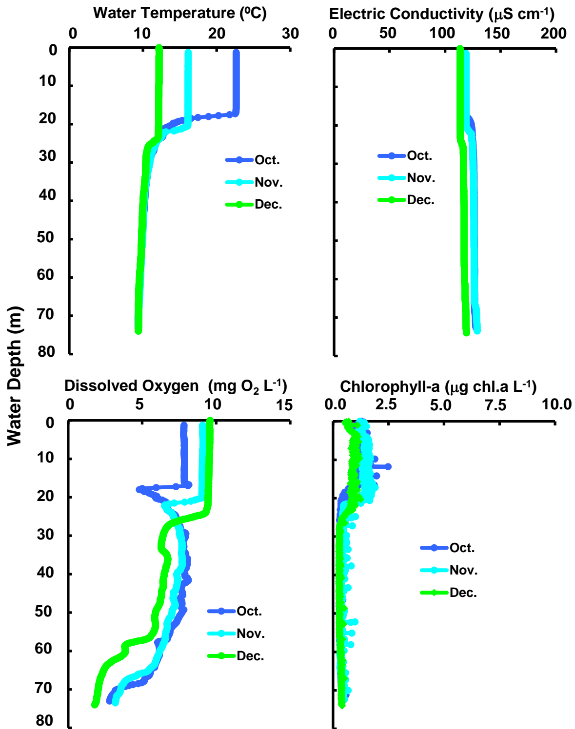
Changes of vertical distribution in water temperature, electric conductivity, dissolved oxygen concn., chlorophyll-a amount at Stn.le-1 in the north basin of Lake Biwa from October to December 2020.
