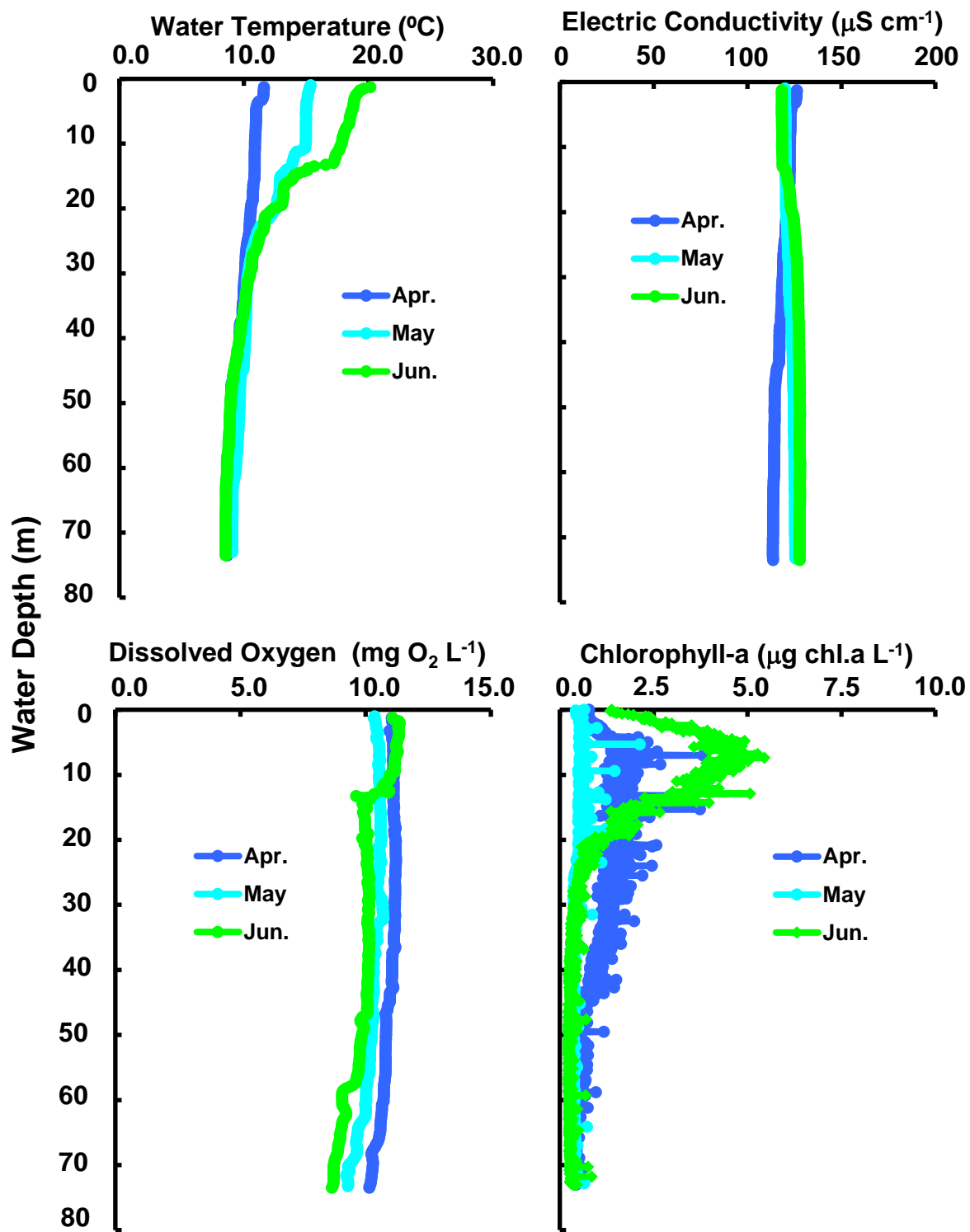
Changes of vertical distribution in water temperature, electric conductivity, dissolved oxygen concn., chlorophyll-a amount at Stn.1e-1 in the north basin of Lake Biwa from April to June 2021.
