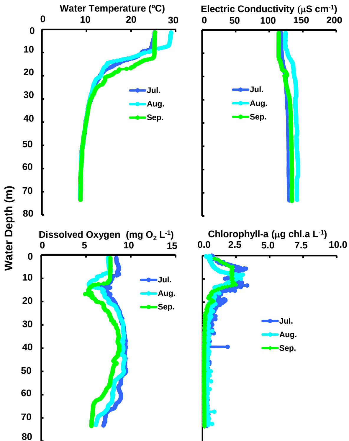
Changes of vertical distribution in water temperature, conductivity, dissolved oxygen concn., chlorophyll-a amount at Stn.le-1 in the north basin of Lake Biwa from July to September 2021.
