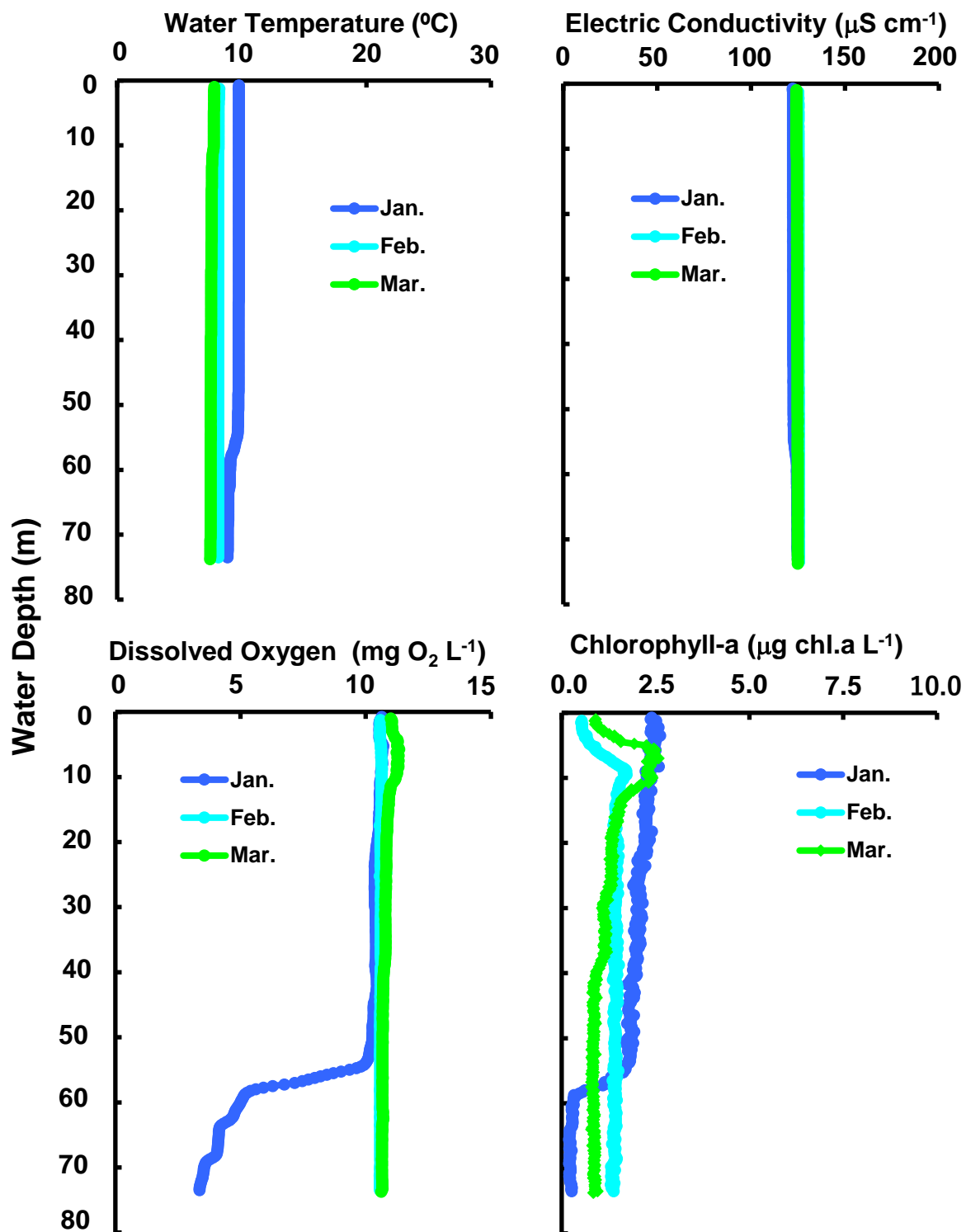
Changes of vertical distribution in water temperature, electric conductivity, dissolved oxygen concn., chlorophyll-a amount at Stn. 1e-1 in the north basin of Lake Biwa from January to March 2022.
