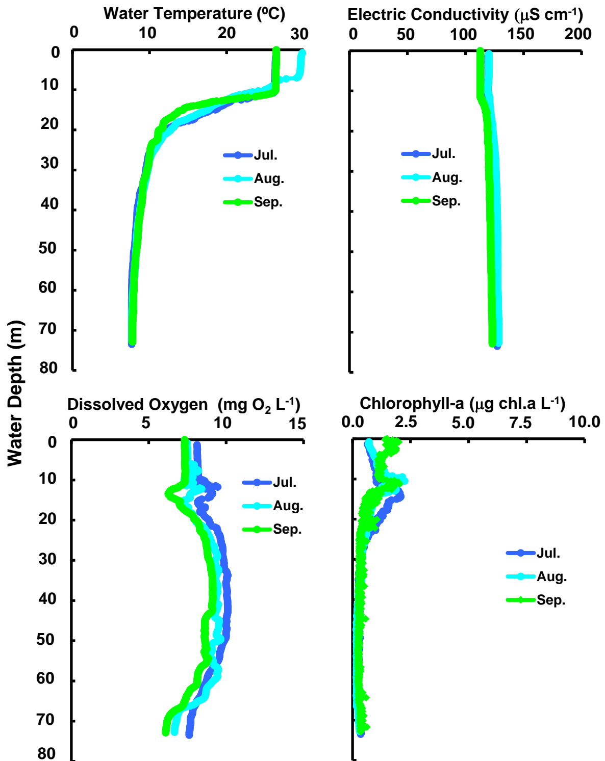
Changes of vertical distribution in water temperature, conductivity, dissolved oxygen concn., chlorophyll-a amount at Stn.le-1 in the north basin of Lake Biwa from July to September 2022.
