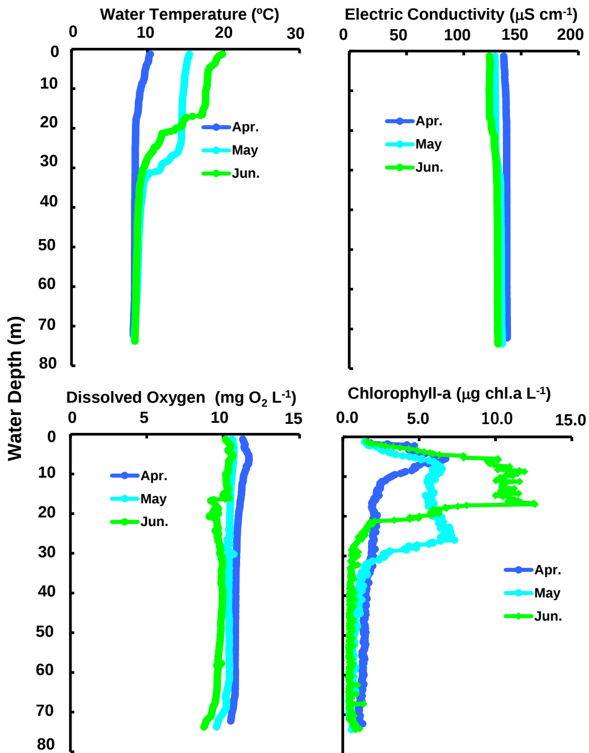
Changes of vertical distribution in water temperature, electric conductivity, dissolved oxygen concn., chlorophyll-a amount at Stn.le-1 in the north basin of Lake Biwa from April to June 2024.
